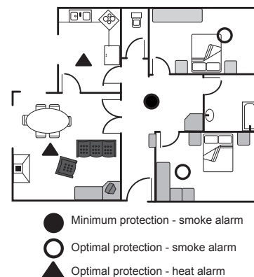
Single-storey house
